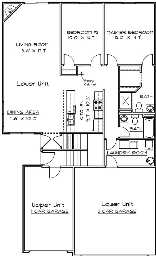
Lower Unit & Garage Layouts
